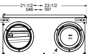
MOTORIZED DAMPER
