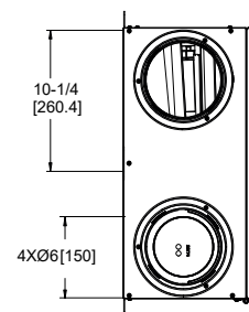
MOTORIZED DAMPER
