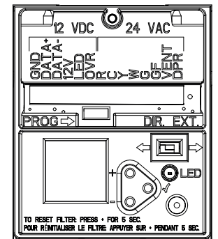
LCD SCREEN AND TERMINAL LOW VOLTAGE CONNECTIONS
