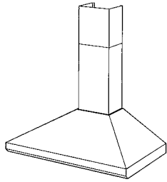
619004 6" Round Duct — Internal Blower 450 CFM, 9.0 Sones 614804 8" Round Duct — Internal Blower 900 CFM, 9.5 Sones 8" Round Duct — External Blower 280 – 1500 CFM
