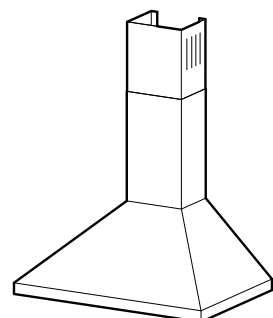
6" Round Duct - Internal Blower 350 CFM, 9 Sones
