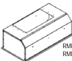
RMIP33 RMIP45 3-1/4" x 10" Duct — Internal Blower 460 CFM, 10.5 Sones 3-1/4" x 14" Duct — External Blower 850 CFM, 10.5 Sones 10" Round Duct — External Blower 280 – 1500 CFM
