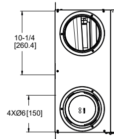
MOTORIZED DAMPER
