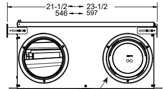
MOTORIZED DAMPER
